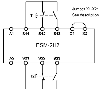
Fig. 1: Wiring of the ESM-2H2.. with a 2-hand push-buttons
