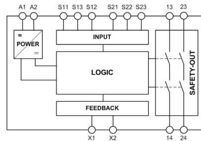
Fig. 1 Block diagram ESM-2H2..
